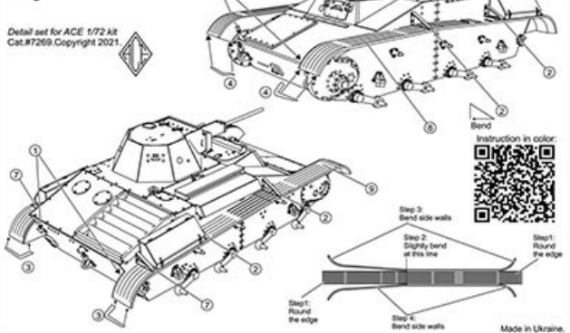
Light Tank T-60 wings
